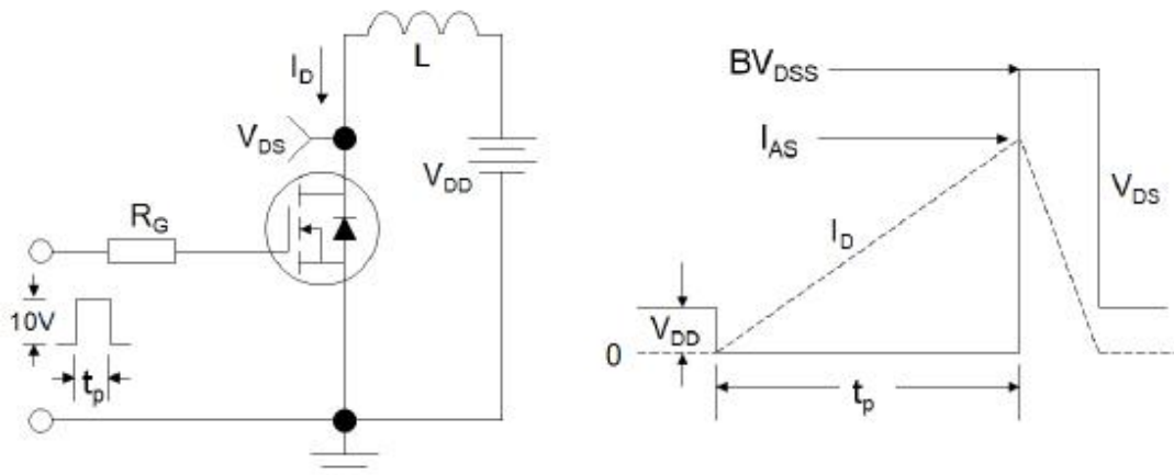
Figure 3:Unclamped Inductive Switching Test Circuit &amp; Waveforms
